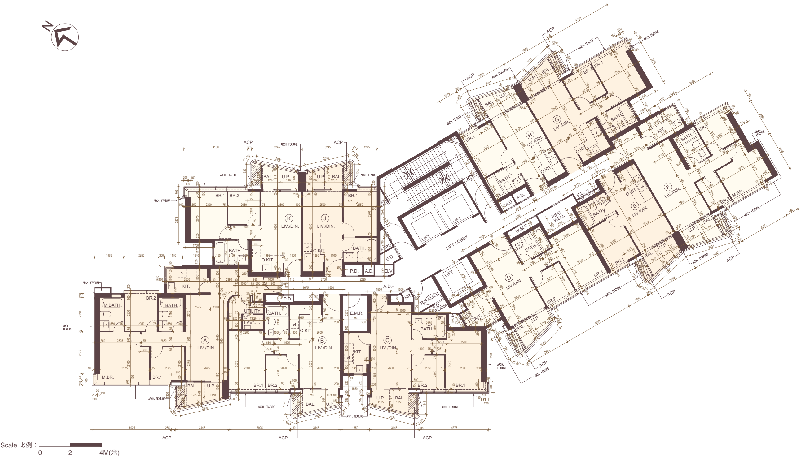
33/F PLAN (Showing the "as-is" condition) 33樓平面圖（顯示「現狀」）
